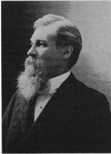
Thomas Chamberlin was noted for his contributions to glaciology and for his part in formulating the Chamberlin-Moulton (planetesimal) hypothesis of the origin of the earth.
