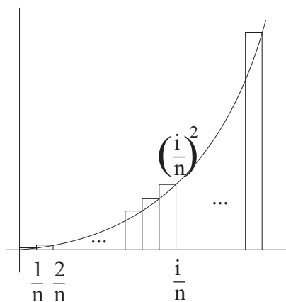
Figure 1: y = x^2
