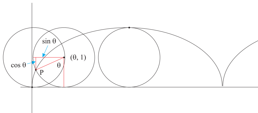
Figure 1: The cycloid.
